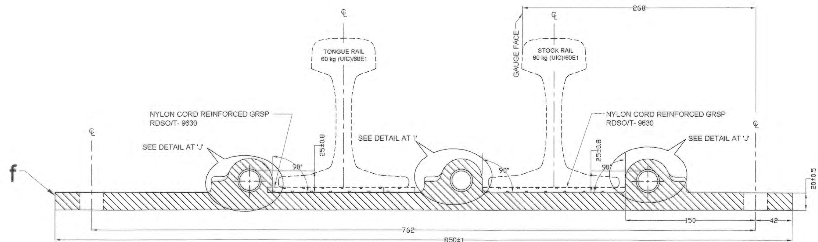
SECTIONAL ELEVATION ON GH
